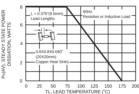
FIG. 5 - STEADY STATE POWER DERTING CURVE
